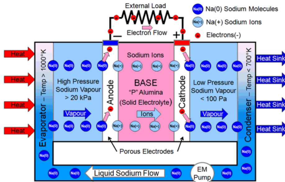
AMTEC Direct Energy Conversion
